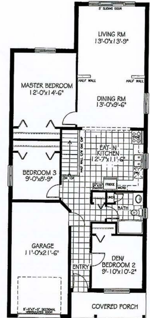
MAIN FLOOR PLAN 'B'
