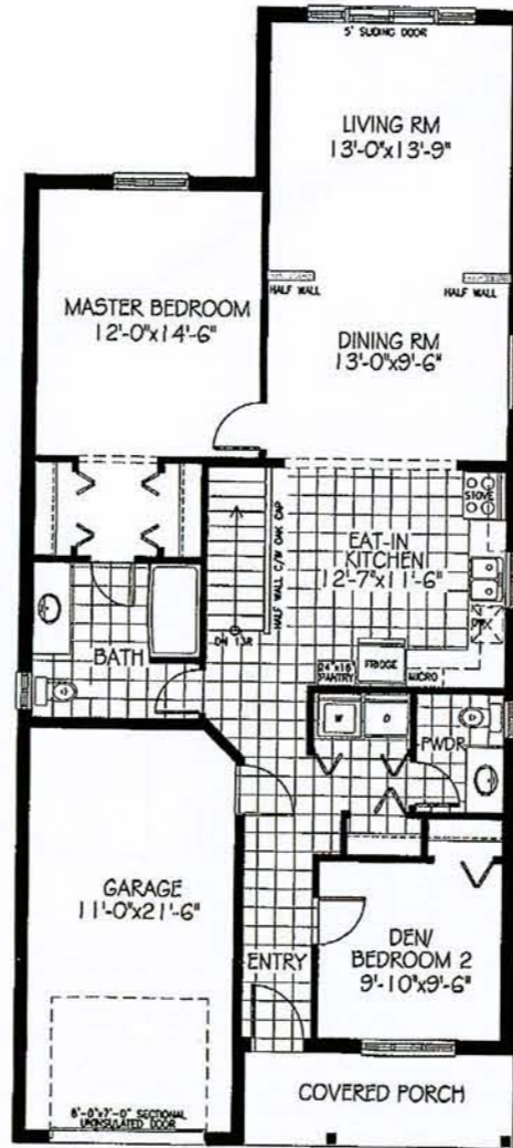
MAIN FLOOR PLAN 'A'
